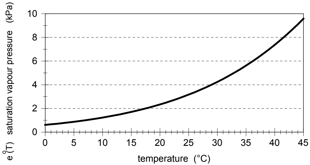
FIGURE 11 Saturation vapour pressure shown as a function of temperature: e^{\circ}(T) curve
